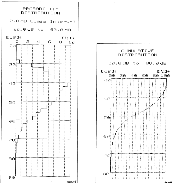
Fig. 10. Examples of plots of amplitude and cumulative distributions
