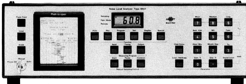
Fig. 1. The Noise Level Analyzer Type 4427
