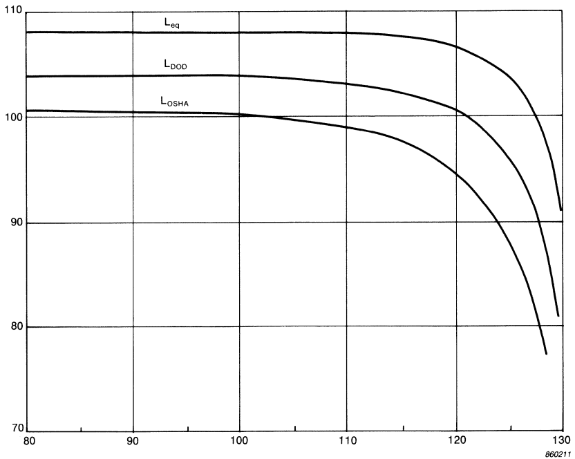
Fig. 19. a) Variation of L_{eq} , L_{DOD} and L_{OSHA} as a function of the threshold level
