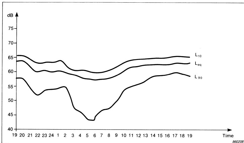
Fig. 13. Variation of hourly L_{eq} , L_{10} and L_{90} over a 24 h period
