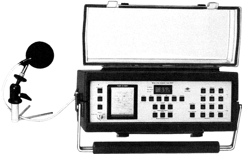
Fig. 7. Use of the Noise Level Analyzer in a Carrying Case KA 2004
