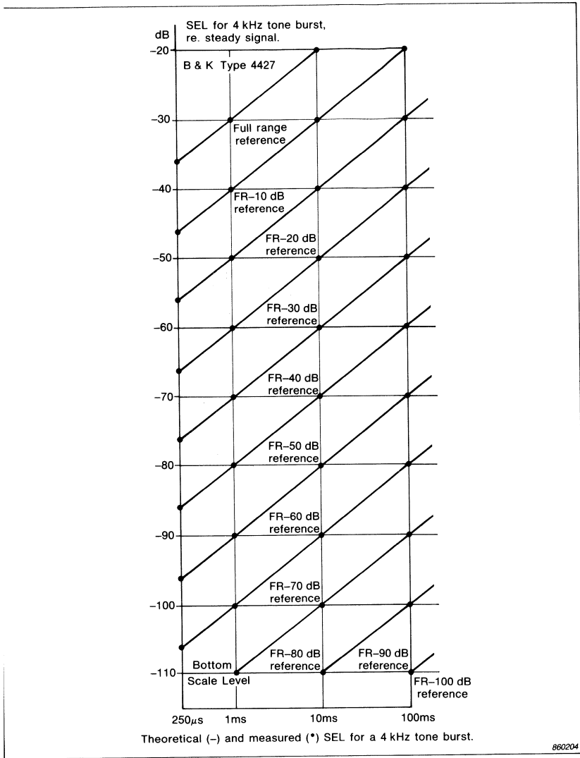
Fig. 3. a) Theoretical and measured sound exposure level for a 4 kHz tone burst
