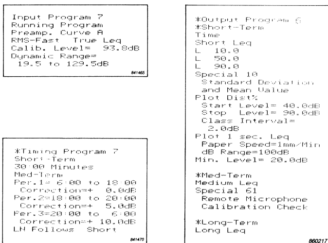
Fig. 6. Examples of user-defined measurement set-ups
