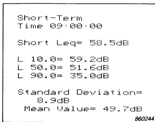
Fig. 12. Example of hourly report
