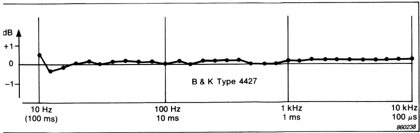
Fig. 4. Error on measured A-weighted pulse duration level
